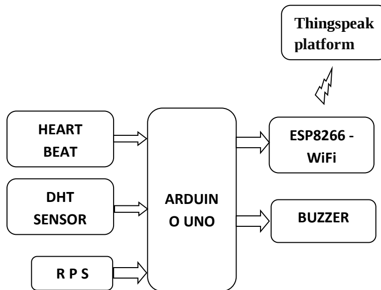
Figure.1 Block Diagram
